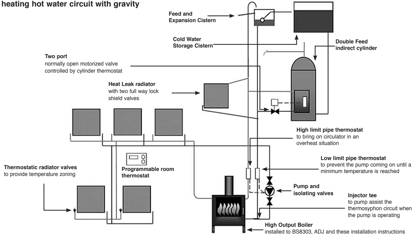
Typical layout of a pumped central heating and hot water circuit
