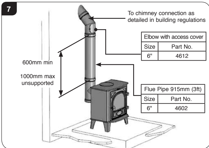
Typical Rear Flue Installation
