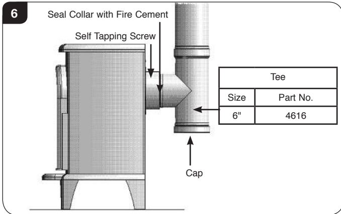
Typical Rear Flue Installation
