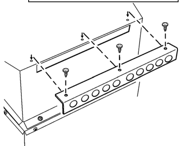
Figure 16. Flue restrictor
