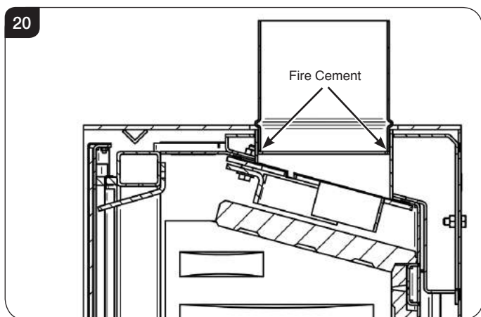
Flue Pipe Installation
