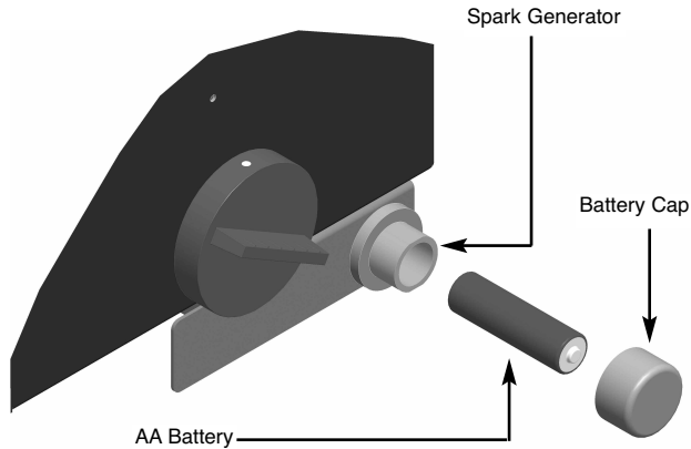
Fig. 6 FITTING THE BATTERY (CONT.)
