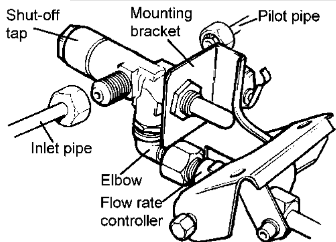
Figure 41. Shut-off tap (Viewed from rear with burner turned over)
