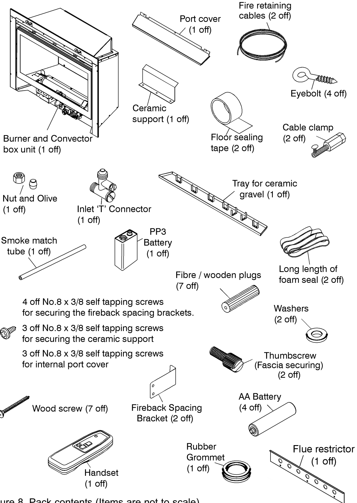
Figure 8. Pack contents (Items are not to scale)
