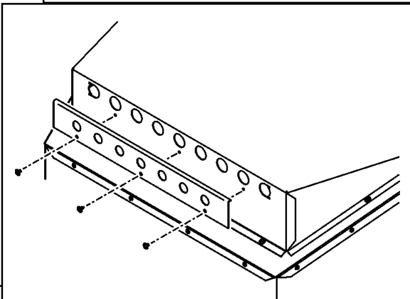
Figure 13B. Flue restrictor
