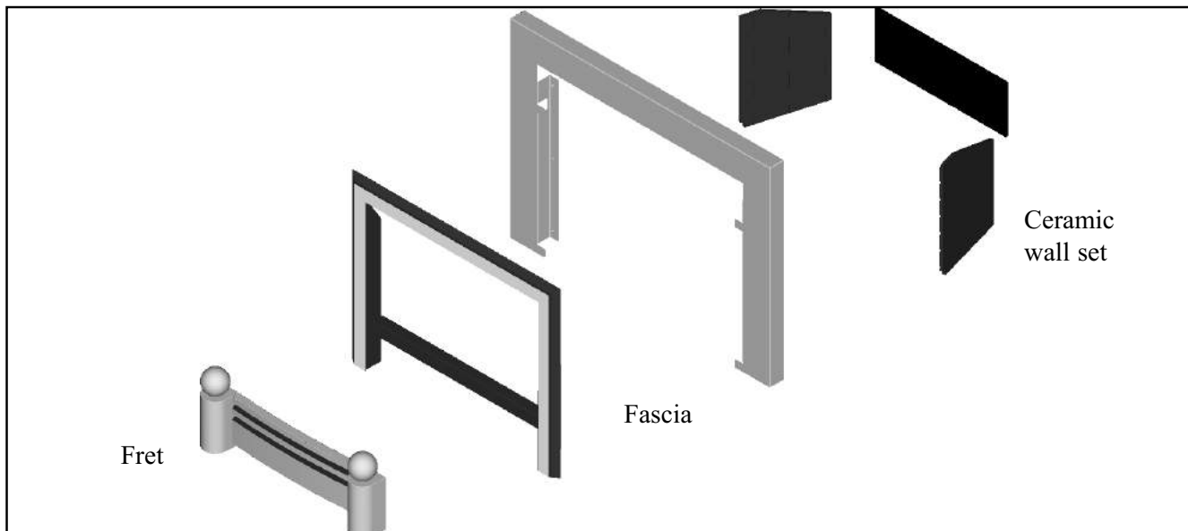
Figure 8A. Blakely fascia - Pack contents continued (Items are not to scale)
