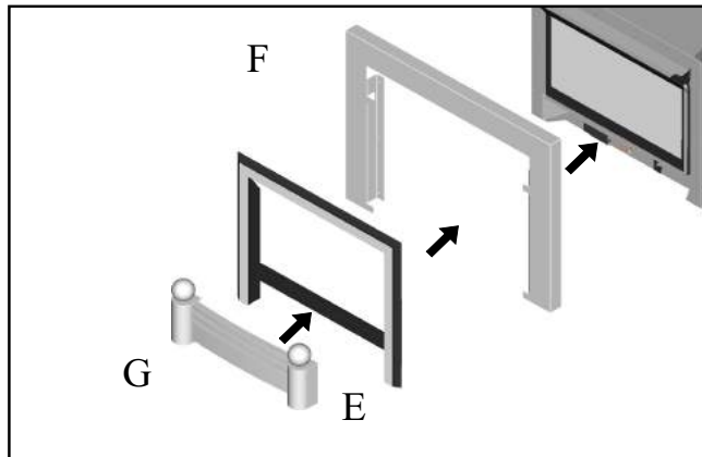
Figure 9. Blakely fascia fitting
