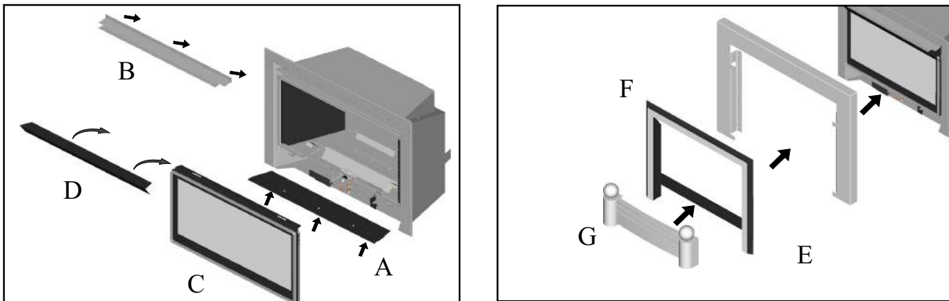
Fig 27 - Fitting Blakely fascia
