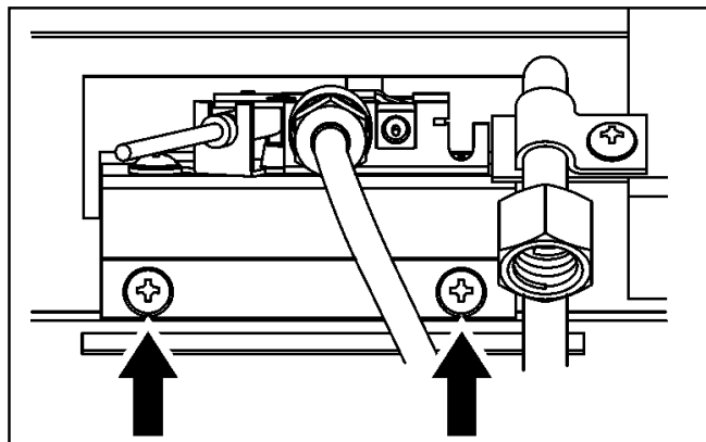
Figure 33. Pilot / pilot bracket assembly removal
