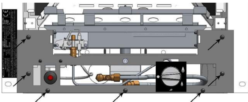
Removal of the manual burner tray
